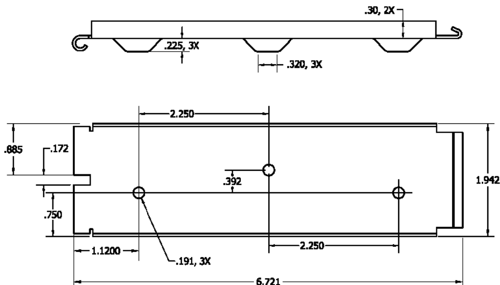
Figure 3-3 Remote Mounting Tray Dimensions
