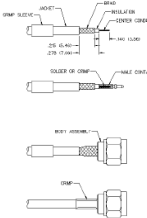
Figure 3-7 Antenna SMA Assembly
