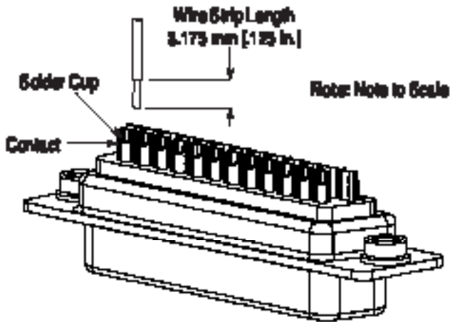
Figure 3-5 J2/J3 Connector Wiring
